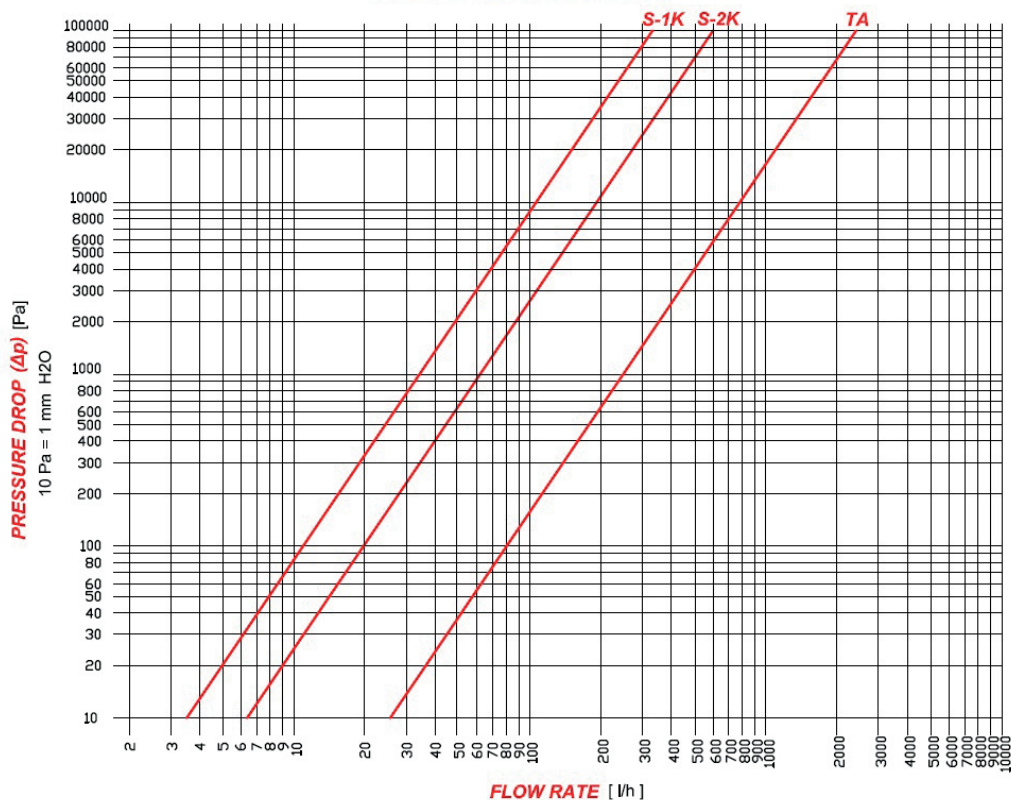
Thermostatic Valve 774 - 3/4"
