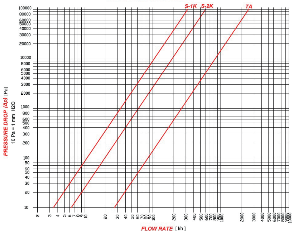
Thermostatic Valve 774 - 3/4"
